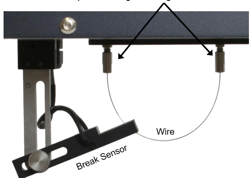
Micro Chucks shown installed in a Model FTX High Speed Rotating Wire Fatigue Tester
